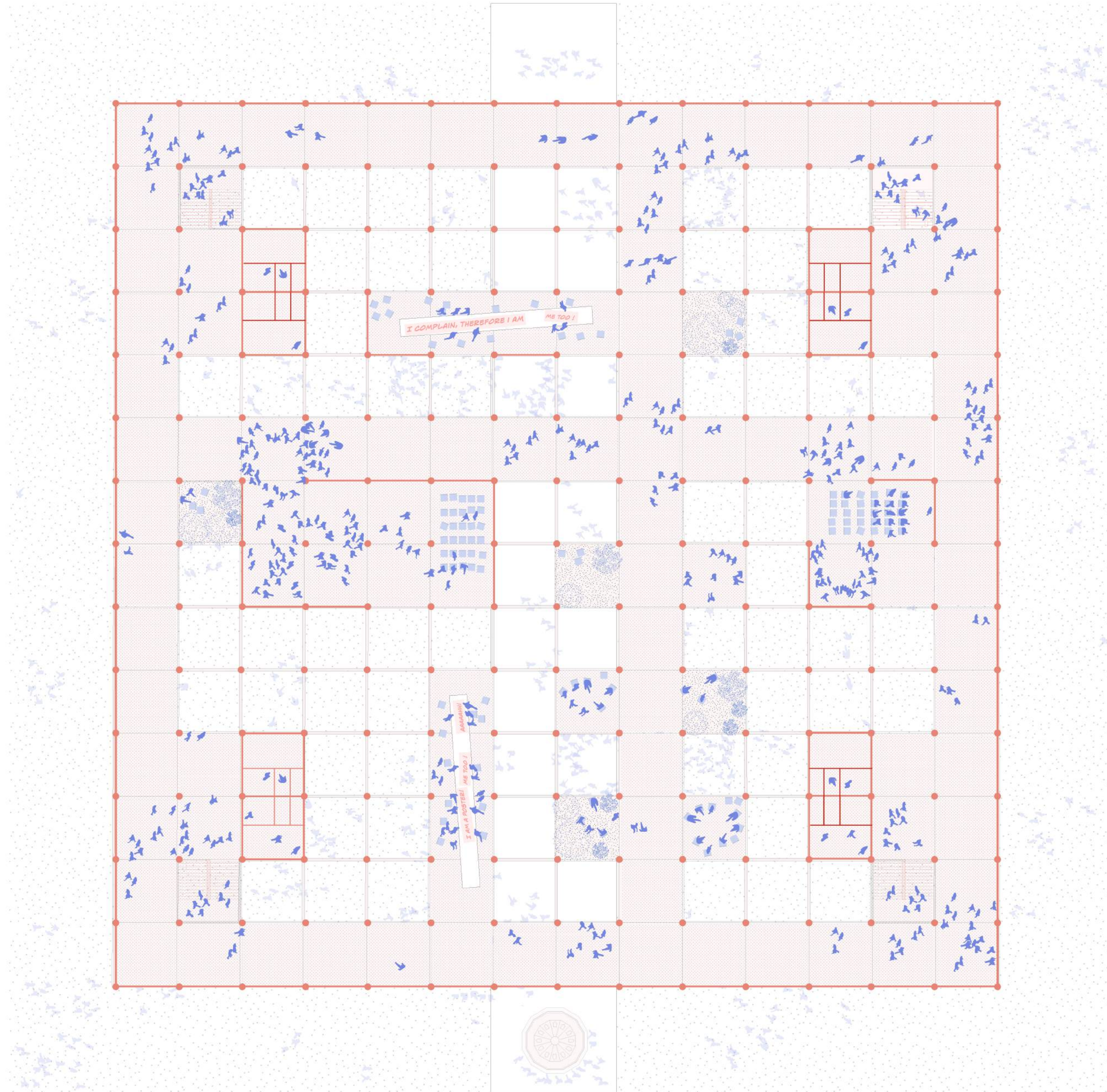
elevated floor plan 1:250
